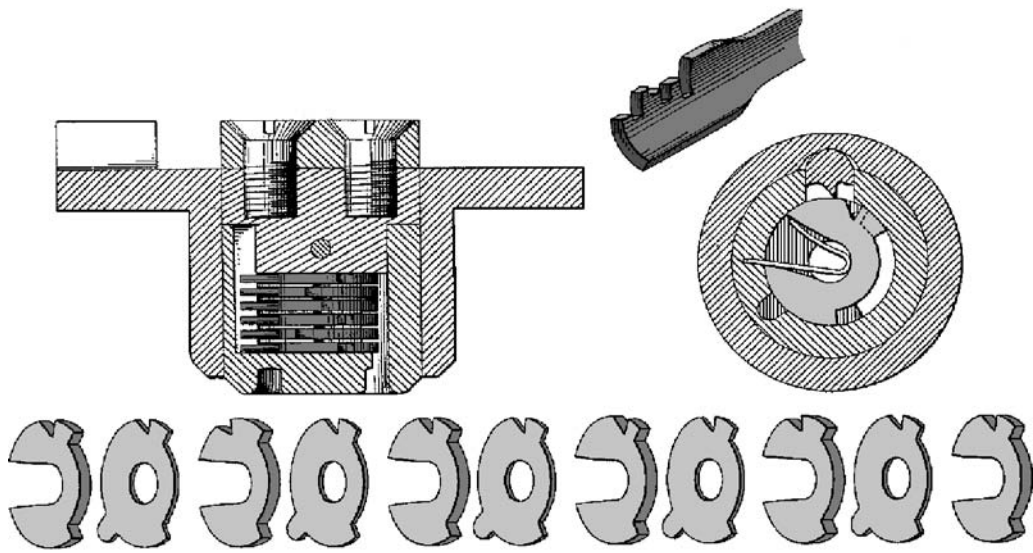
Figure 4.6: An early form of disc-tumbler side-bar lock from 1901 (US patent 688,070 by W. G. Denn).
