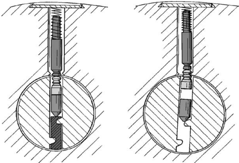
Figure 2.24: R. Hucknall's pick-proof pin (1971 US patent 3,762,193).
