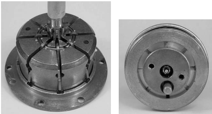
Figure 5.103: Operation of Monopole core: key aligns lever gates with gap at rear.
