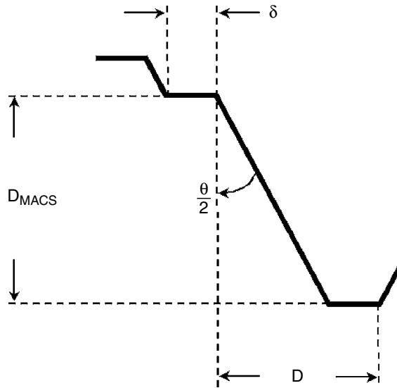
Figure 2.11: Notation for adjacent pins with maximum difference in depth of cut.
