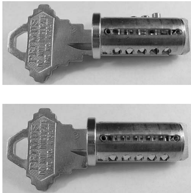
Figure 4.118: Operation of Schlage Primus core with side-bar removed: key aligns finger pins.
