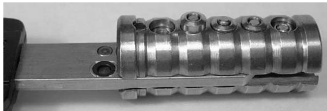
Figure 2.191: Key partially inserted: movable insert not yet in contact with pin 1.
