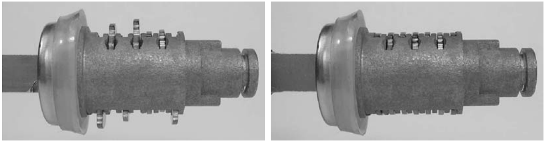
Figure 7.10: Operation of Commodore double-sided wafer lock.
