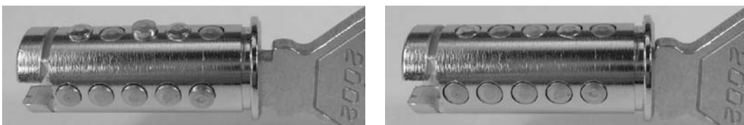
Figure 2.123: KESO 2002 core with key at various stages of insertion.
