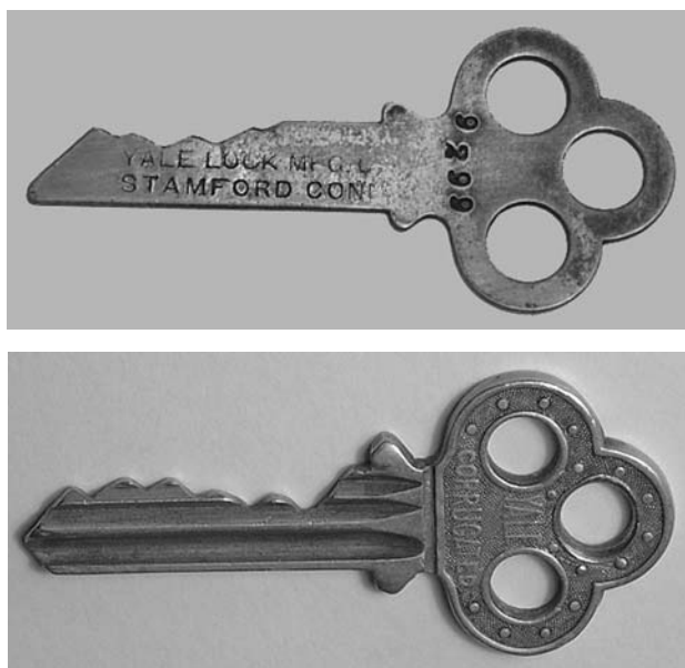
Figure 2.2: (Top) Early Yale flat pin-tumbler key. (Bottom) Yale corrugated key.
