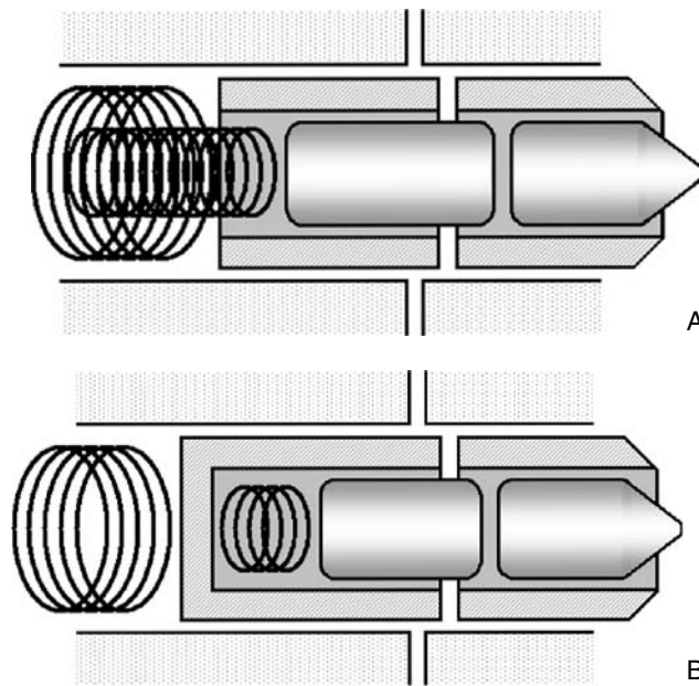
Figure 2.181: Two different types of concentric pin-tumbler mechanisms.
