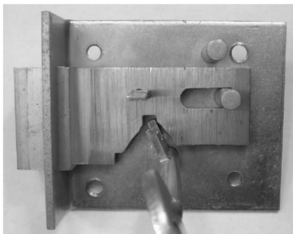
Figure 5.1: Ross 100 lever lock with levers removed. Key contacts talon of bolt in either direction.
